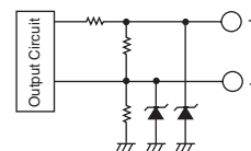
Output Circuit
