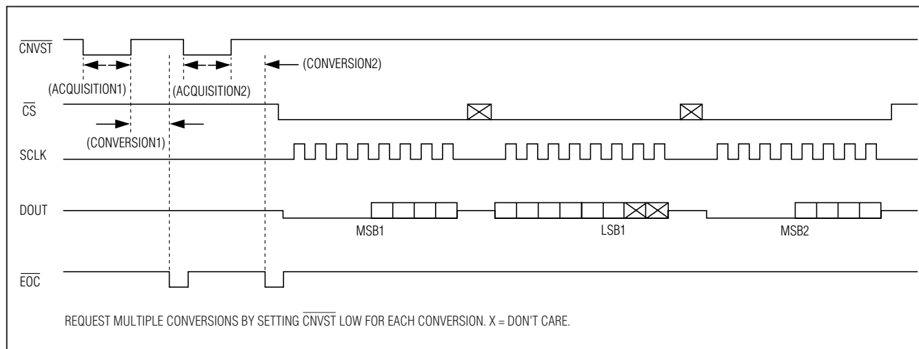
Figure 5. Clock Mode 01
