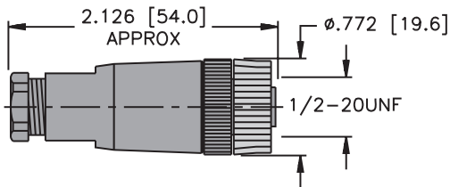
Female Connector
