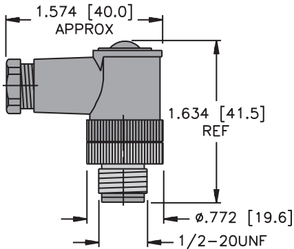
Male Connector
