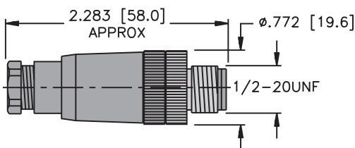
Male Connector
