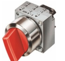
Selector switch, 2 switch positions, standard version, 50°
