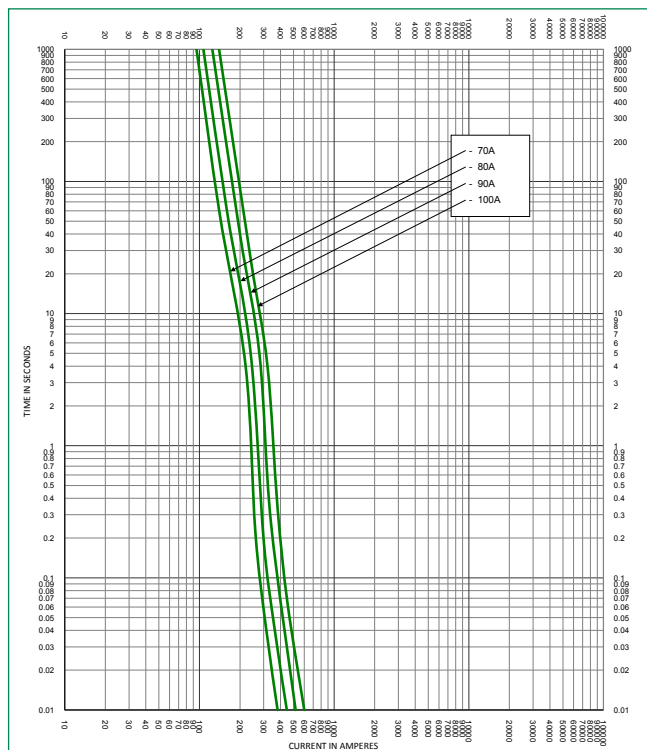
Time Current Curve JLLN (70–100 A)
