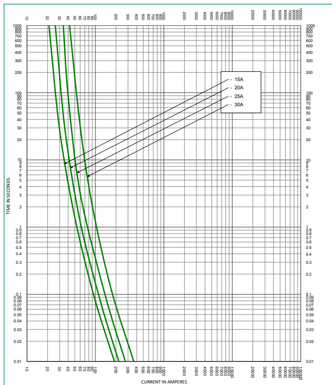
Time Current Curve JLLN (15–30 A)
