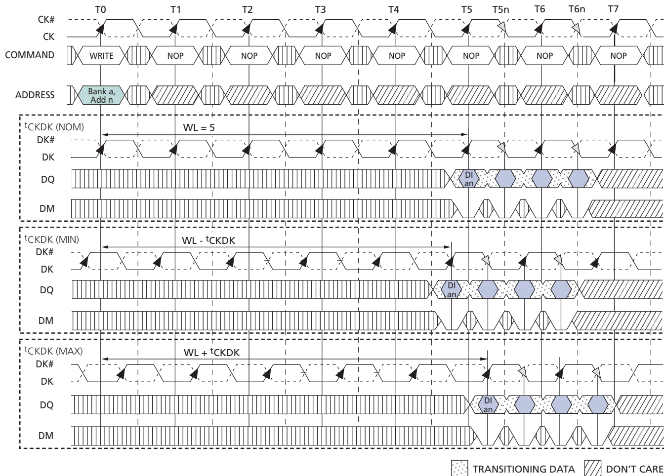
Figure 29: WRITE Burst
