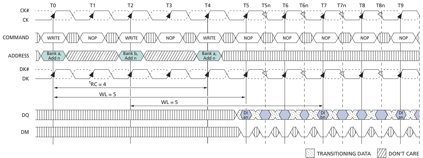
Figure 30: Consecutive WRITE-to-WRITE
