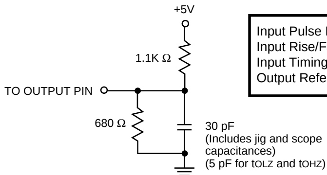
FIGURE 3. AC TEST CONDITIONS
