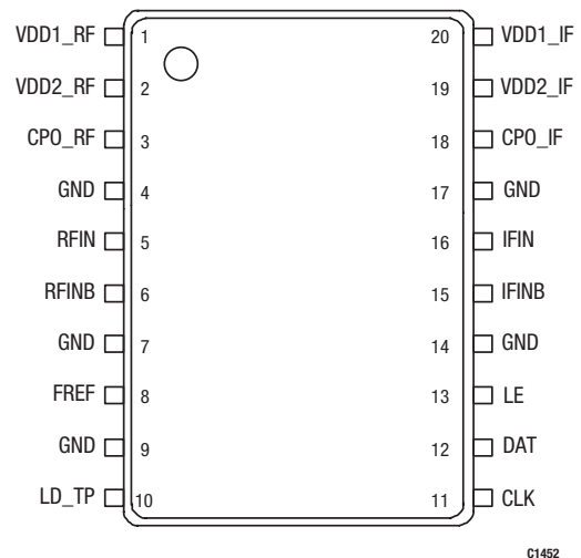
Figure 1. SKY74038 Pinout – 20-Pin TSSOP (Top View)
