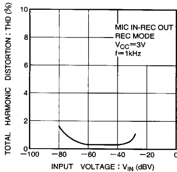
Fig. 8 Distortion vs. input voltage
