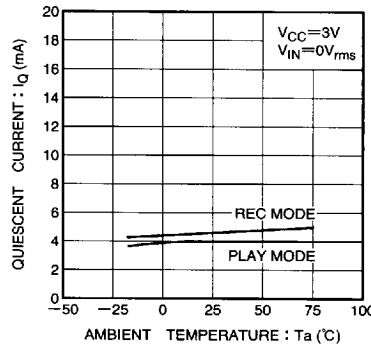
Fig. 12 Quiescent current vs. ambient temperature
