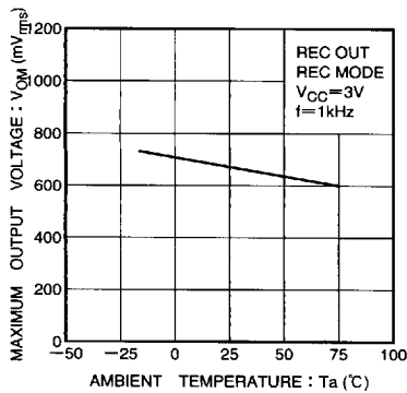
Fig. 11 Output voltage vs. ambient temperature
