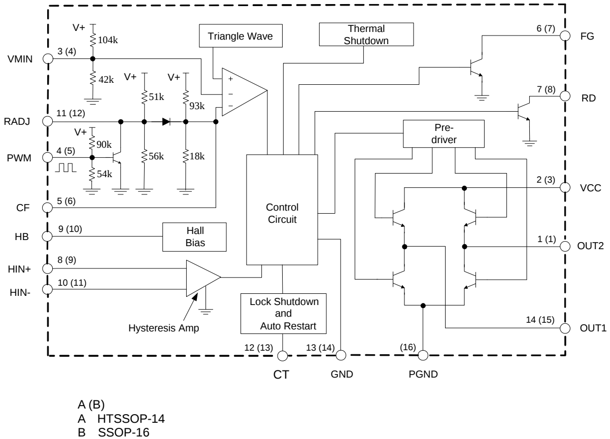
Figure 3. Functional Block Diagram of AM4962
