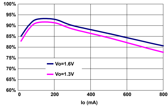
FIGURE 3. EFFICIENCY ( V_{\text{in}} = 3.6\text{V} )
