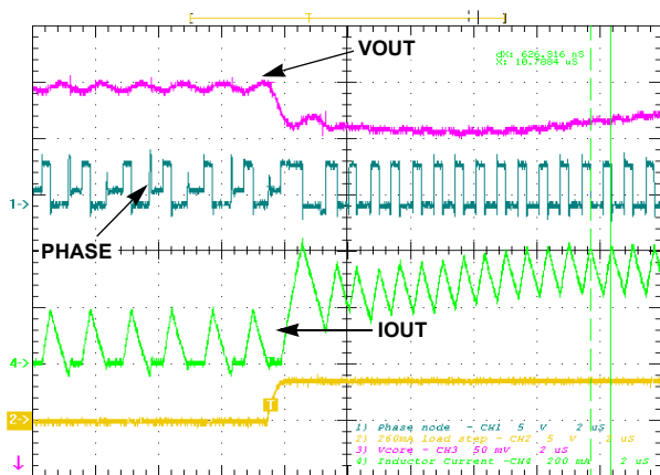
50mA to 260mA load step on VOUT. Top: Output voltage, 50mV/DIV; Phase node, 5V/DIV; Inductor current, 200mA/DIV, 2 \mu\text{s} /DIV
