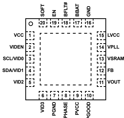
ISL6271A (4x4 QFN) TOP VIEW
