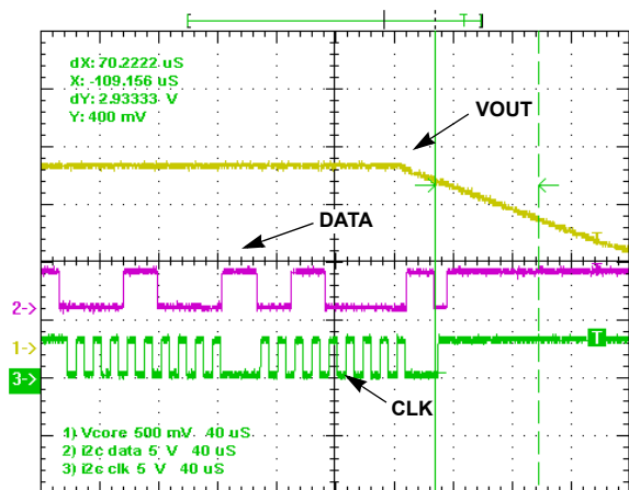
FIGURE 8. TYPICAL I 2 C COMMUNICATION
