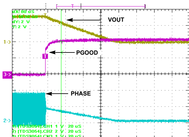
Forced PGOOD fault. Converter operating in CCM at 420mA prior to applying a 320mA transient step. This pushes the regulator beyond the overcurrent threshold of 700mA. The phase node three-states and follows Vout to 0V. 20μs/DIV
