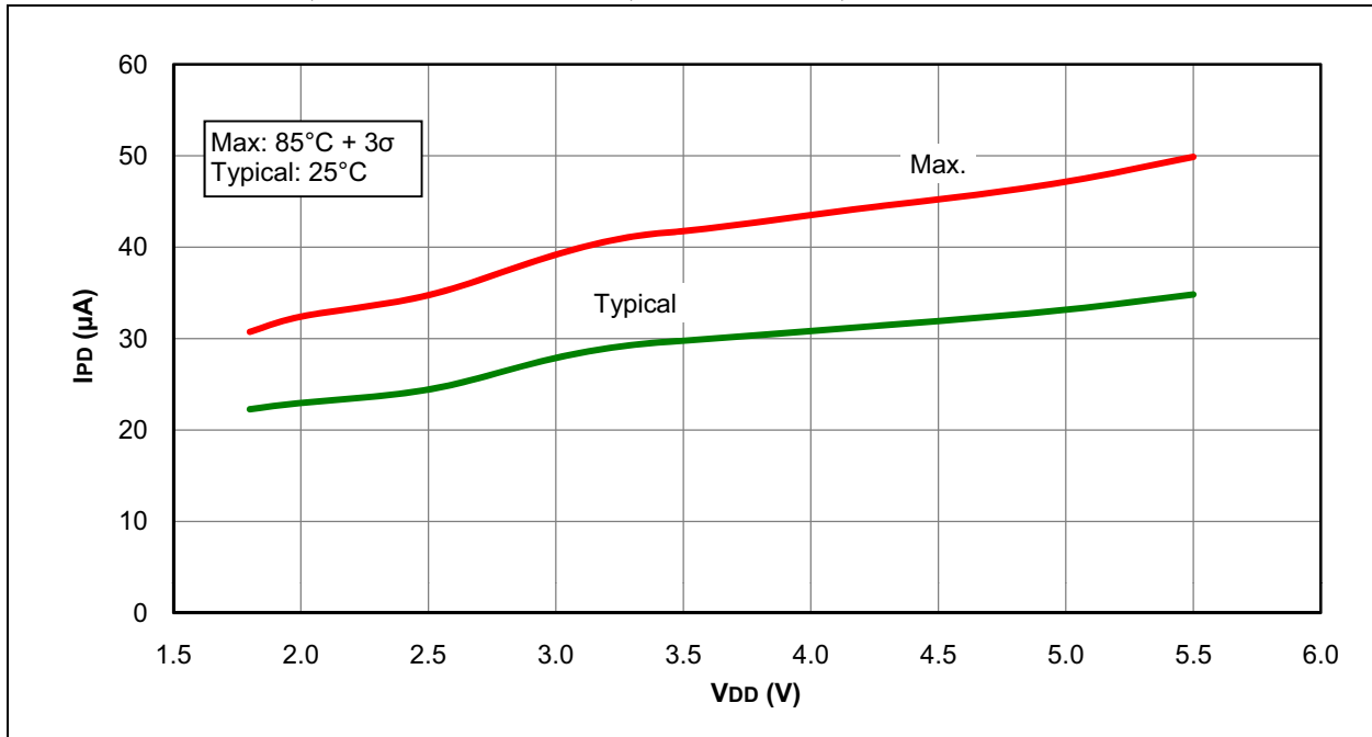
FIGURE 31-40: I_{PD} , TIMER1 OSCILLATOR, F_{osc} = 32 kHz, PIC16F1946/47 ONLY
