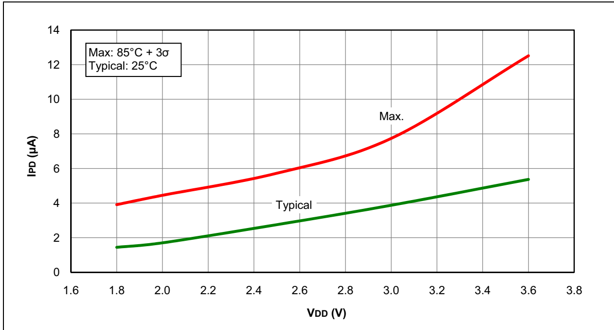
FIGURE 31-39: I_{PD} , TIMER1 OSCILLATOR, F_{osc} = 32 kHz, PIC16LF1946/47 ONLY
