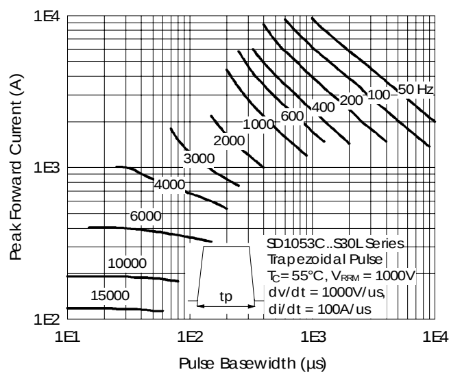
Fig. 39 - Frequency Characteristics
