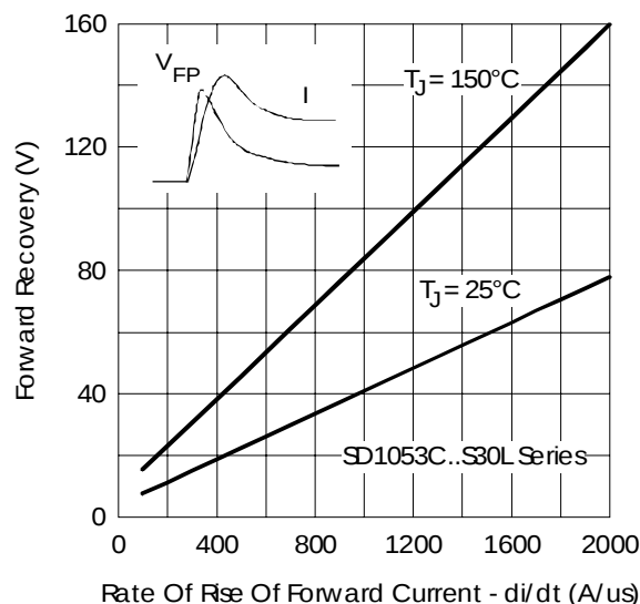
Fig. 21 - Typical Forward Recovery Characteristics
