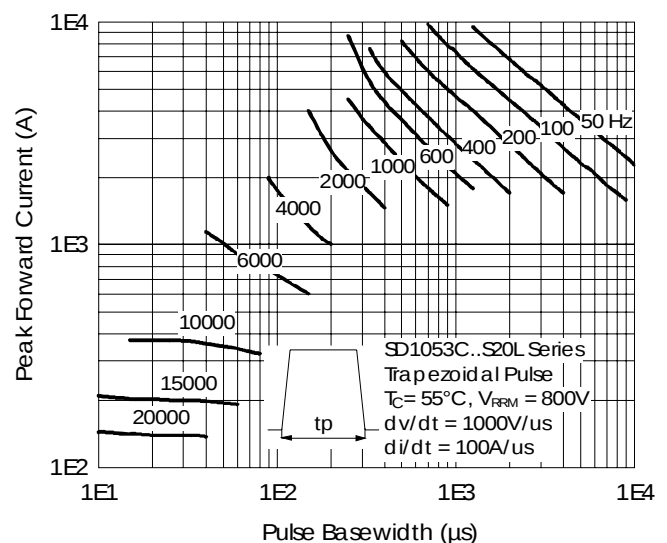
Fig. 33 - Frequency Characteristics
