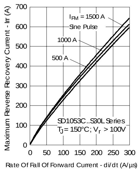
Fig. 27 - Recovery Current Characteristics
