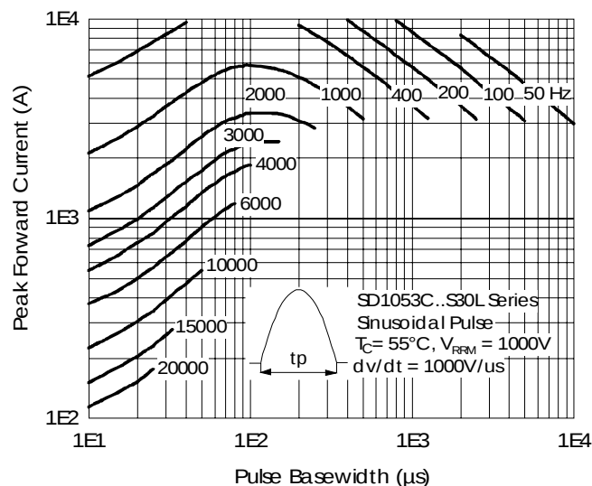
Fig. 35 - Frequency Characteristics
