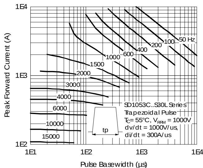
Fig. 37 - Frequency Characteristics
