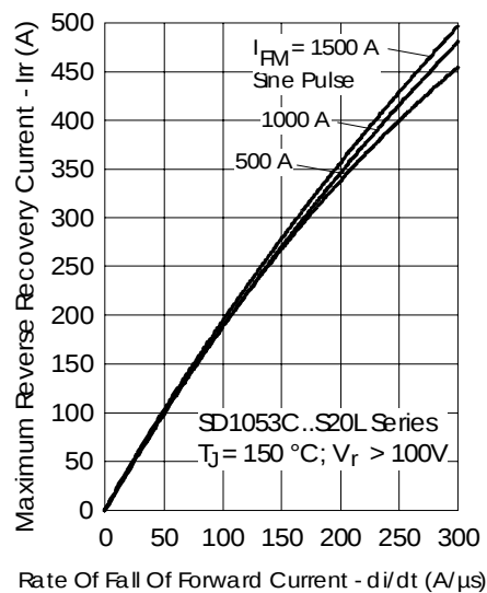
Fig. 24 - Recovery Current Characteristics
