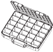
25 inserts 568-030 H=80, W=415, D=330
