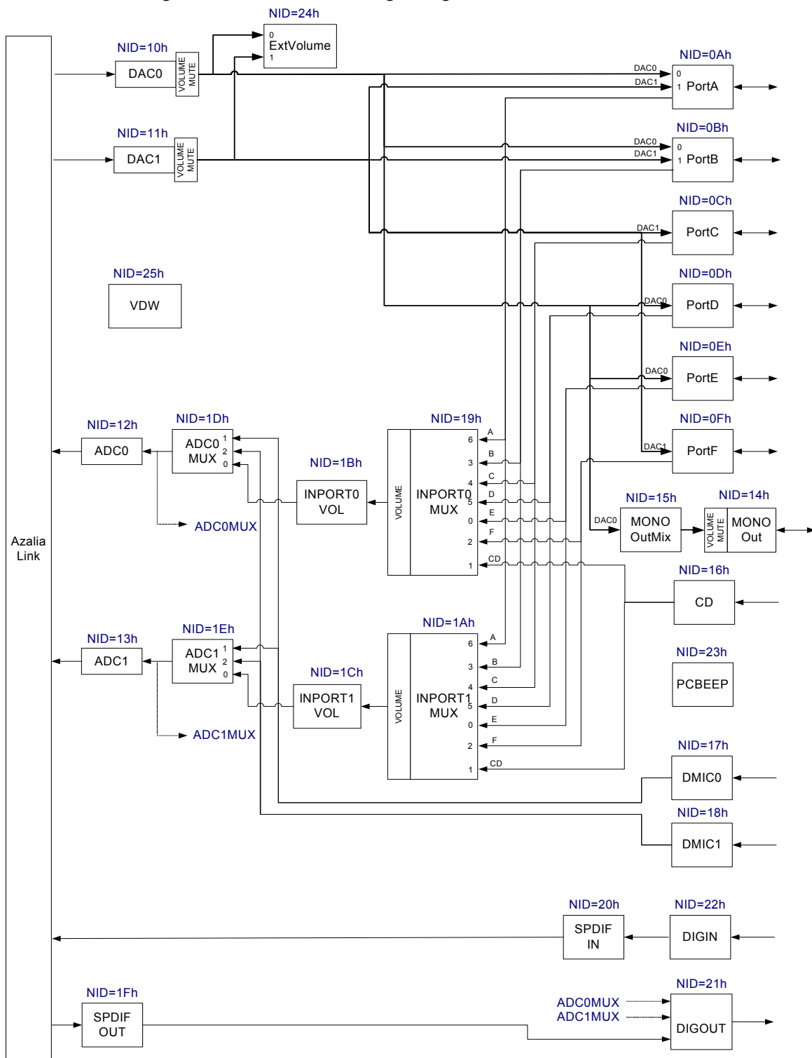
Figure 6. STAC9204/9205 Widget Diagram
