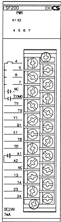
CS1W-SF200
