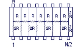
R/2R Ladder CTS Schematic 7
