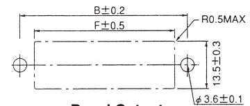
Panel Cutout
