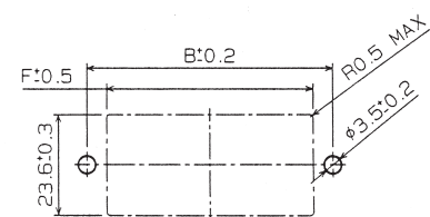
Panel Cutout
