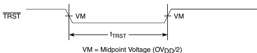
Figure 46. \overline{TRST} Timing Diagram
