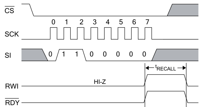
Figure 29. Software RECALL Cycle [26]
