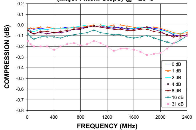
COMPRESSION @ INPUT POWER=+24dBm (Major Atten. Steps) @ +25°C
