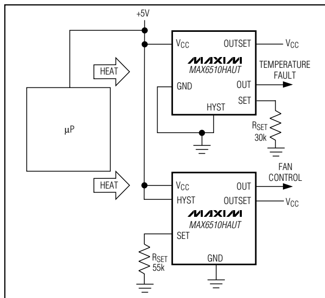
Figure 6. Low-Power, High-Reliability, Fail-Safe Temperature Monitor
