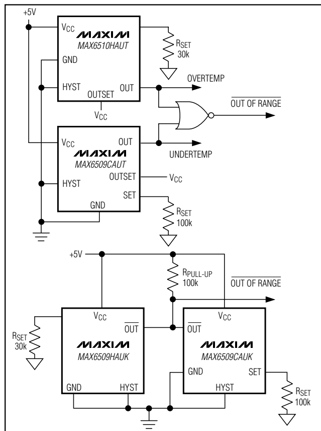
Figure 5. Temperature-Window Detector
