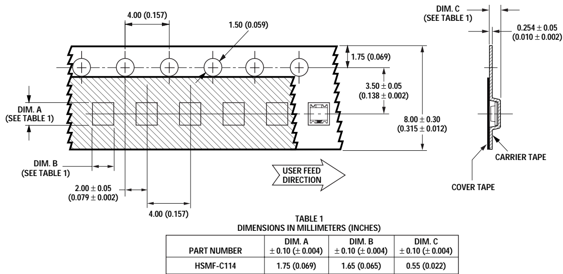
Figure 12. Tape dimensions.
