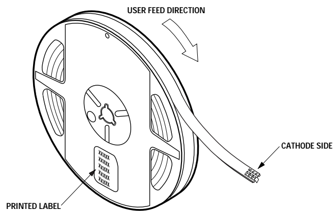
Figure 10. Reeling orientation.
