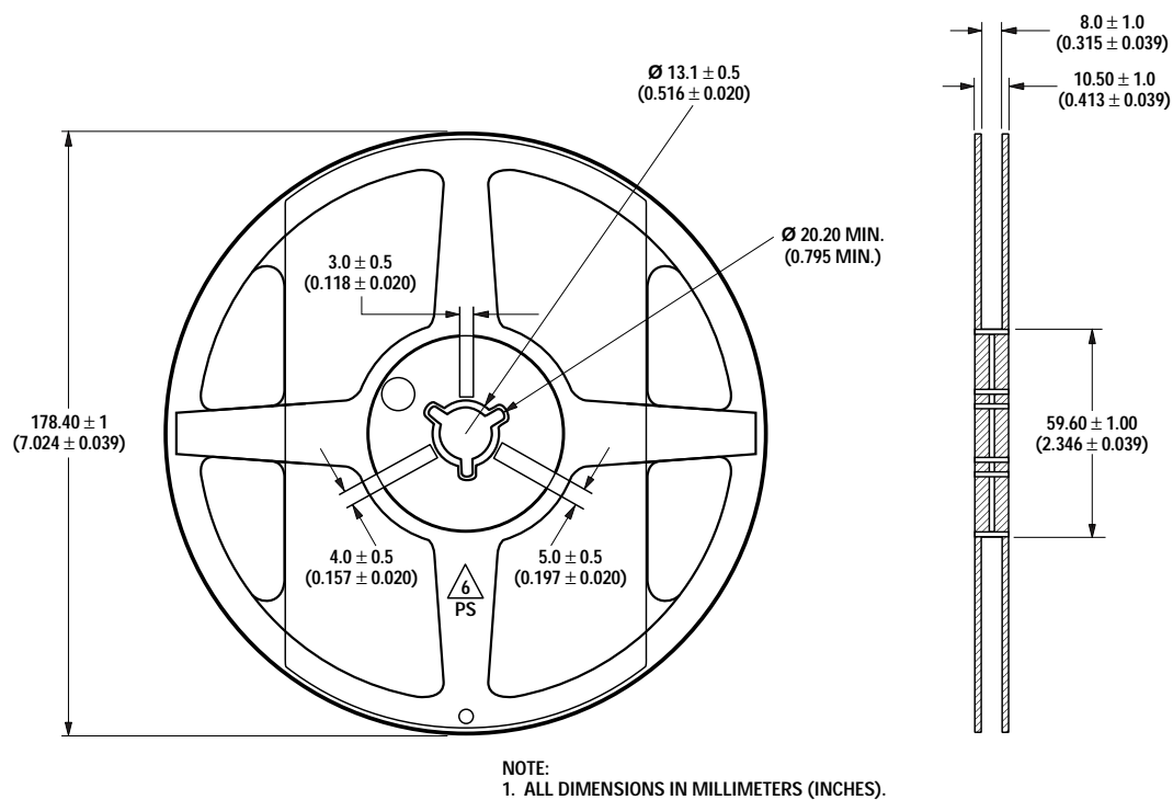
Figure 11. Reel dimensions.
