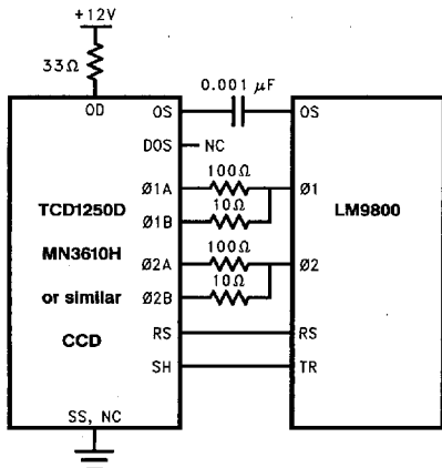
FIGURE 35. CCD Interface Example
