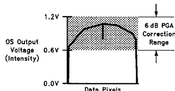
FIGURE 31. CCD Input Signal In Range
