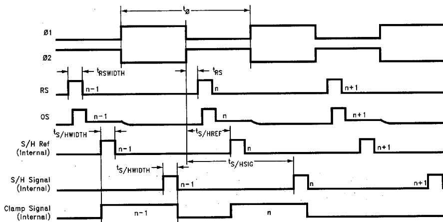
FIGURE 7. CCD Timing
