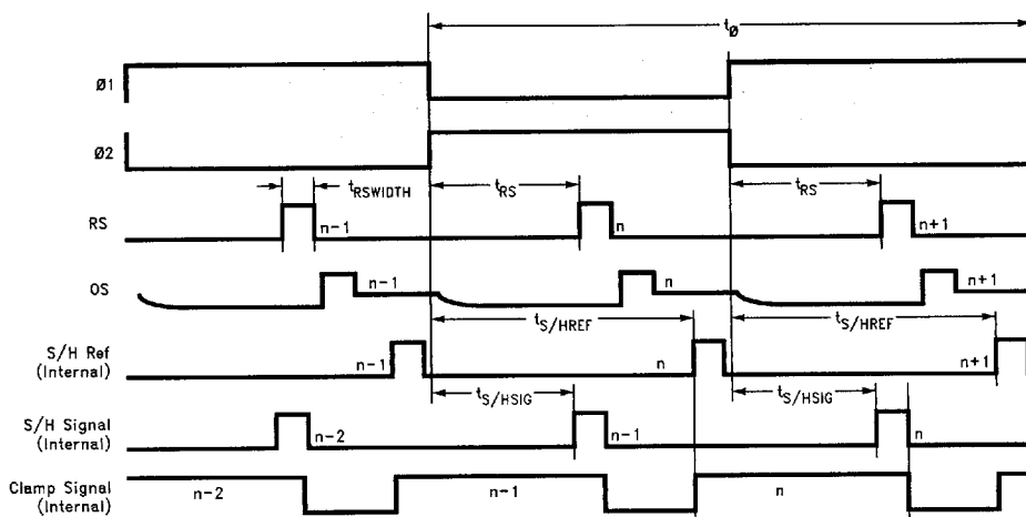
FIGURE 8. CCD Timing (Even/Odd CCDs)
