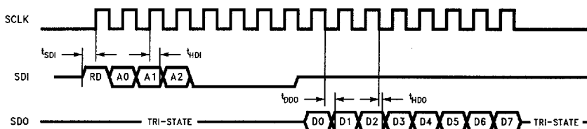
FIGURE 14c. Configuration Register Read Timing with \overline{CS} Continuously Low (16-bit Word)
