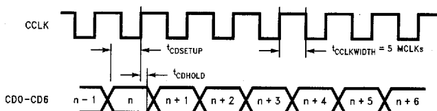
FIGURE 10. Coefficient Data Timing
