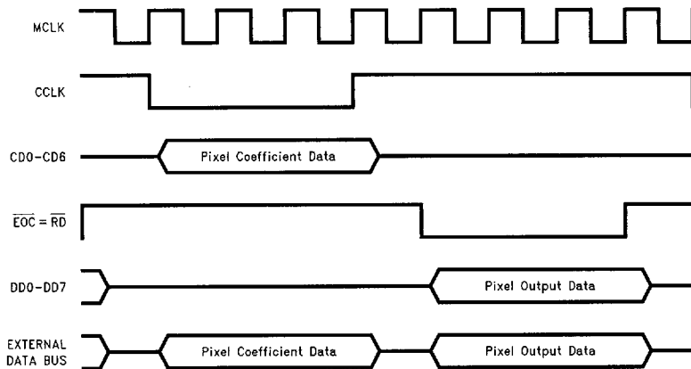
FIGURE 12. Data Timing (Output and Coefficient Data Sharing Same Bus)
