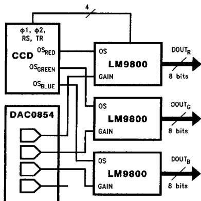
FIGURE 30. Parallel Output CCD, Three LM9800s
