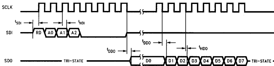
FIGURE 14d. Configuration Register Read Timing with \overline{CS} Continuously Low (Two 8-bit bytes)
