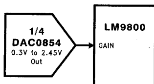
FIGURE 26. GAIN Control with DAC
