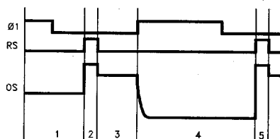
FIGURE 27. CDS
