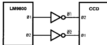
FIGURE 37. \phi 1 and \phi 2 After Inversion
