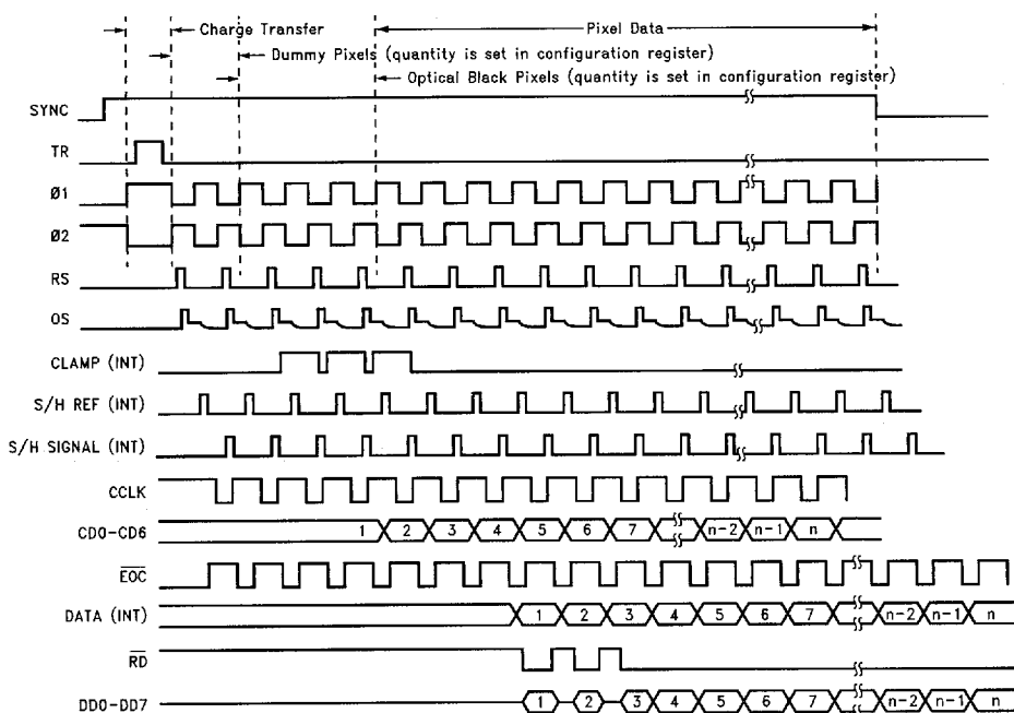
FIGURE 1. Line Scan Timing Overview
