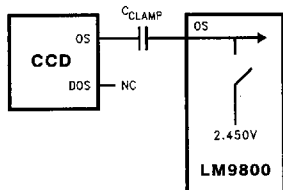
FIGURE 23. OS Clamp Capacitor and Internal Clamp
