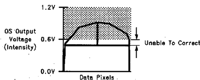
FIGURE 33. CCD Input Signal Too Weak
