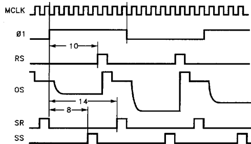
FIGURE 36. Typical Even/Odd Timing
