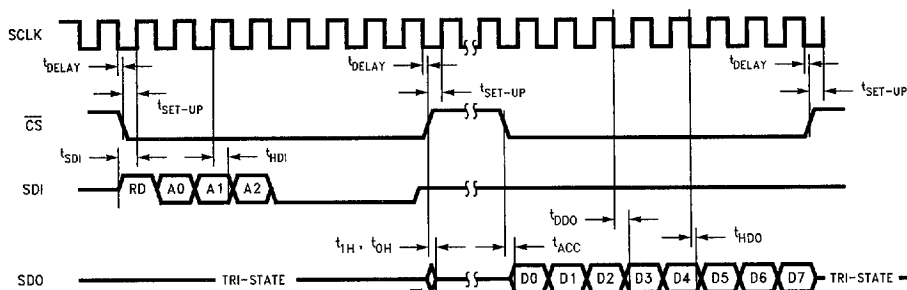
FIGURE 16c. Configuration Register Read Timing using \overline{CS} , Continuous SCLK (16-bit Word)
