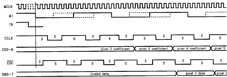
FIGURE 20. SR = 15 (RS Even)
