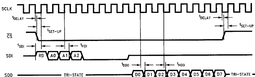
FIGURE 16c. Configuration Register Read Timing using \overline{CS} , Continuous SCLK (16-bit Word)
