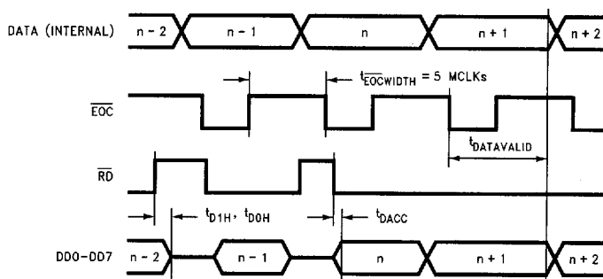
FIGURE 11. Output Data Timing
