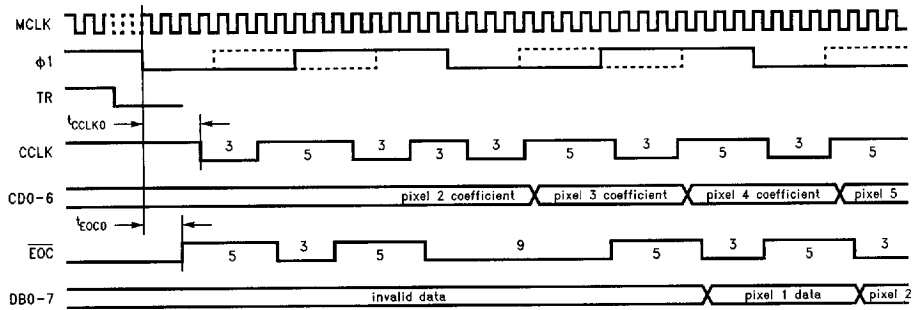
FIGURE 19. SR = 13 or 14 (RS Even), SR = 14 or 15 (RS Odd)
