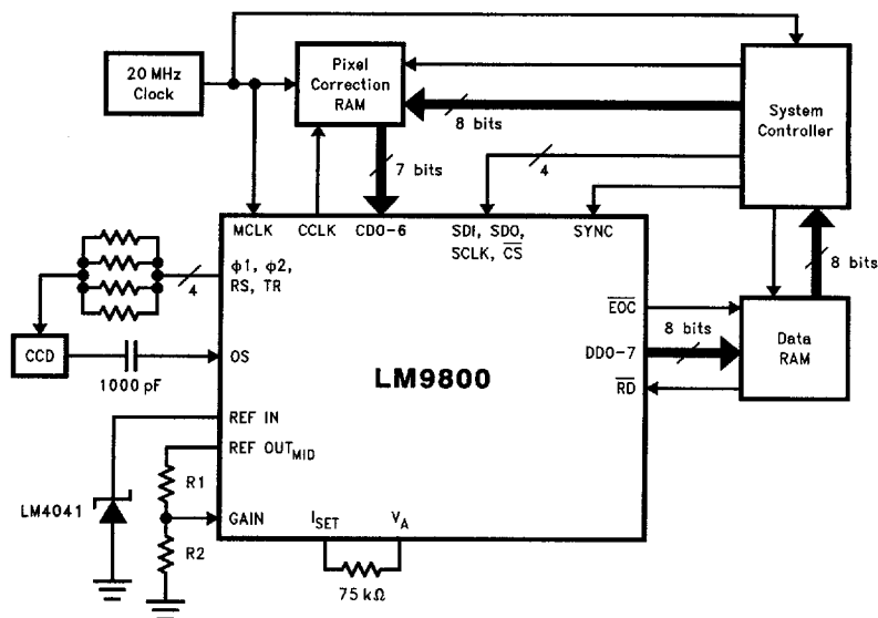
FIGURE 21. LM9800 System Block Diagram
