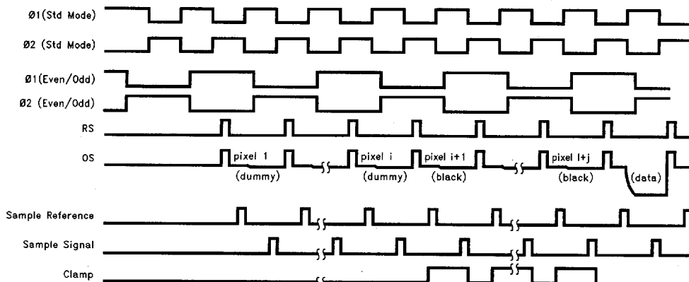
FIGURE 9. Dummy Pixel and Optical Black Pixel Timing
