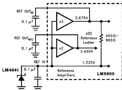
FIGURE 22. Voltage Reference Generation
