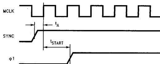
FIGURE 3. Timing for Start of Line Scan
