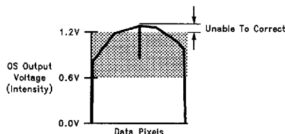
FIGURE 32. CCD Input Signal Too Strong
