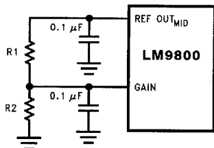
FIGURE 25. GAIN Control with Voltage Divider
