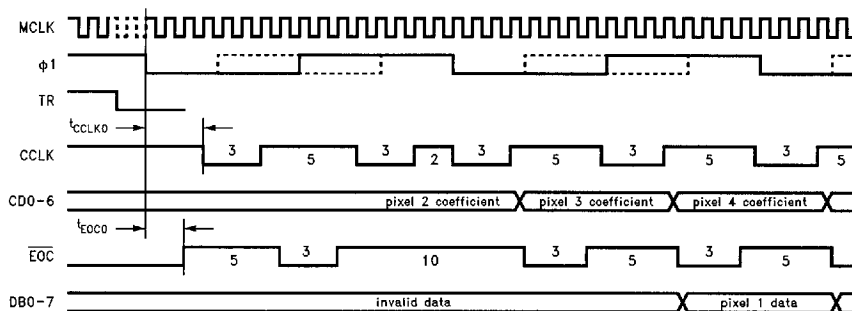
FIGURE 17. SR = 0 through 10 (RS Even), SR = 0 through 11 (RS Odd)
