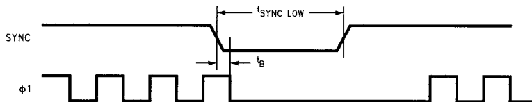
FIGURE 4. Timing for End of Line/Start of Next Line
