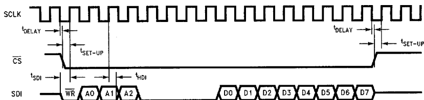
FIGURE 16a. Configuration Register Write Timing using \overline{CS} , Continuous SCLK (16-bit Word)
