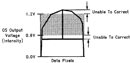
FIGURE 34. CCD Input Signal Range Too Wide
