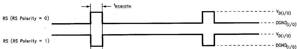
FIGURE 6. RS Pulse Polarity
