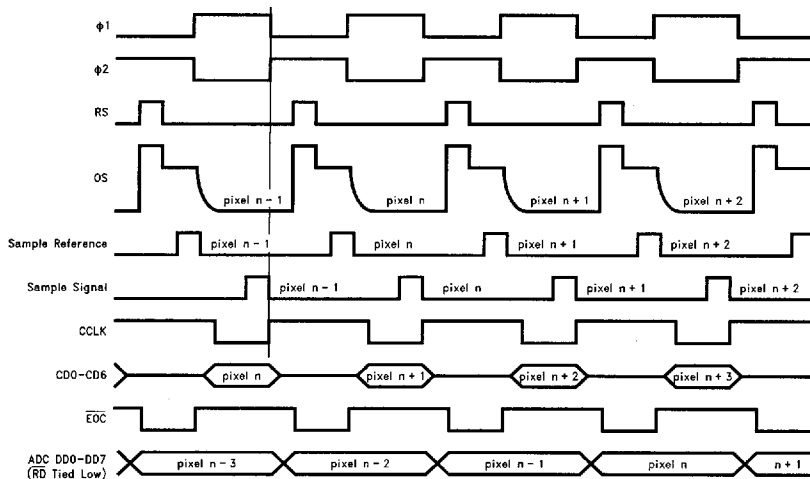
FIGURE 2. Pixel Pipeline Timing Overview
