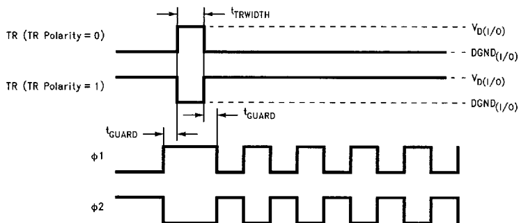
FIGURE 5. TR Pulse
