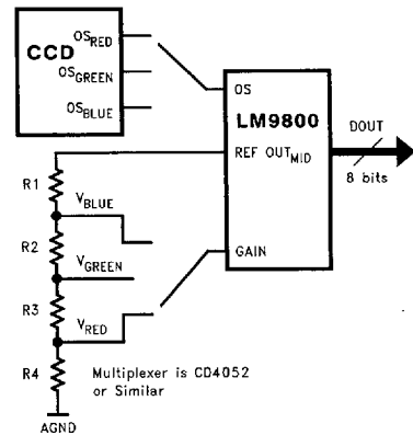
FIGURE 29. Parallel Output CCD, One LM9800
