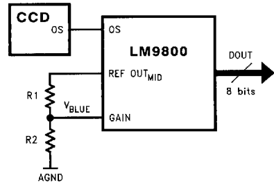
FIGURE 28. Sequential RGB Output CCD
