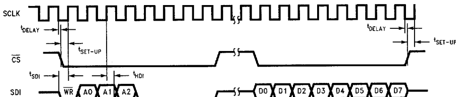
FIGURE 16b. Configuration Register Write Timing using \overline{CS} , Continuous SCLK (Two 8-bit bytes)
