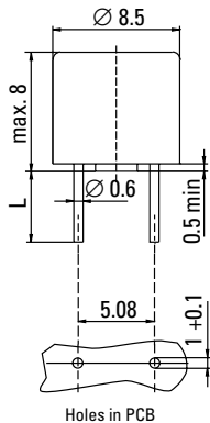
Dimensions (mm)
