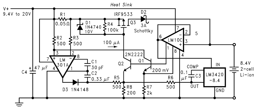
Figure 32. Low Drop-Out Constant Current/Constant Voltage 2-Cell Charger
