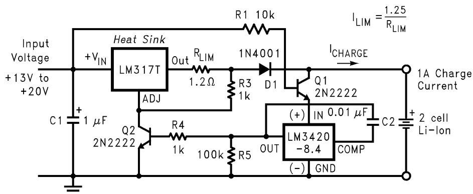
Figure 1. Typical Constant Current/Constant Voltage Li-Ion Battery Charger
