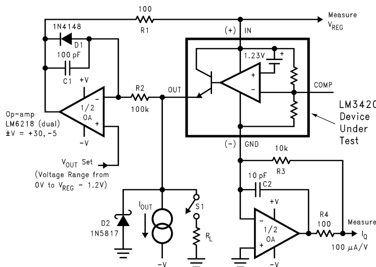
Figure 27. LM3420 Test Circuit
