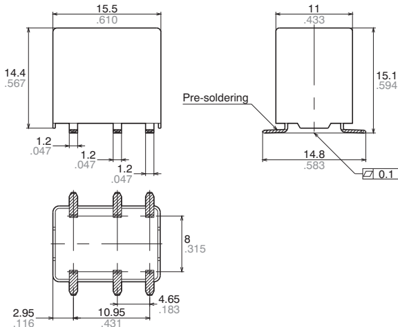
External dimensions
