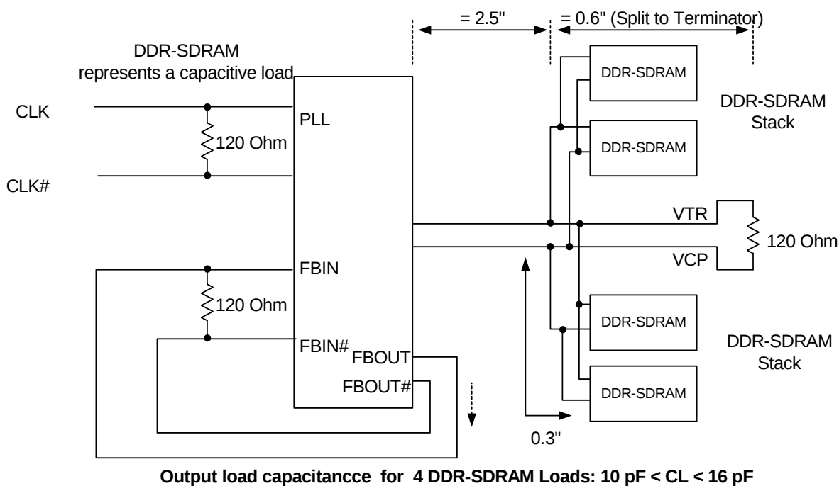
Figure 5. Clock Structure # 1
