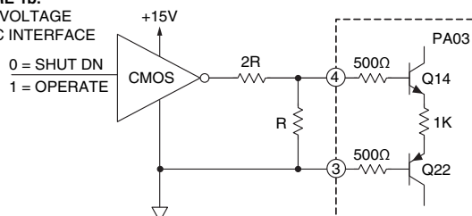
FIGURE 1c. THERMALLY ACTIVATED SHUTDOWN
