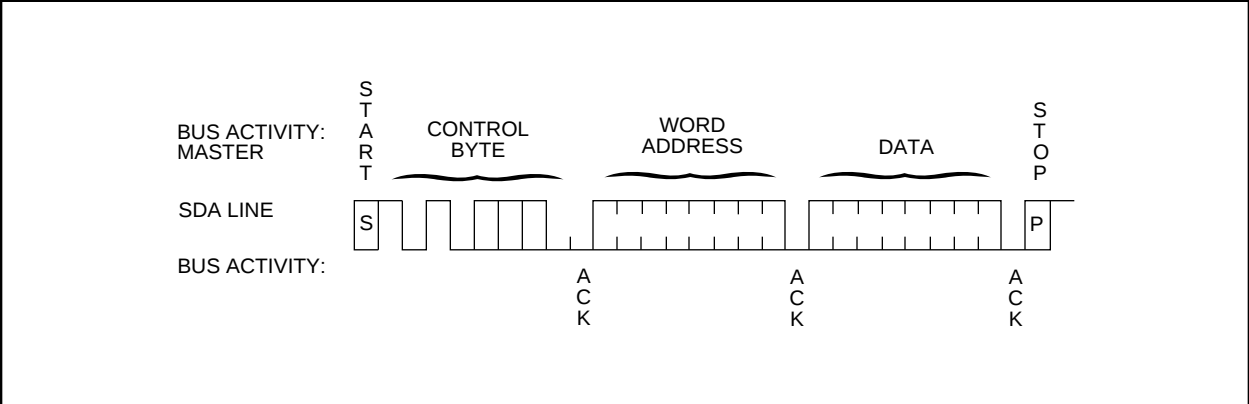
FIGURE 5-1: BYTE WRITE
