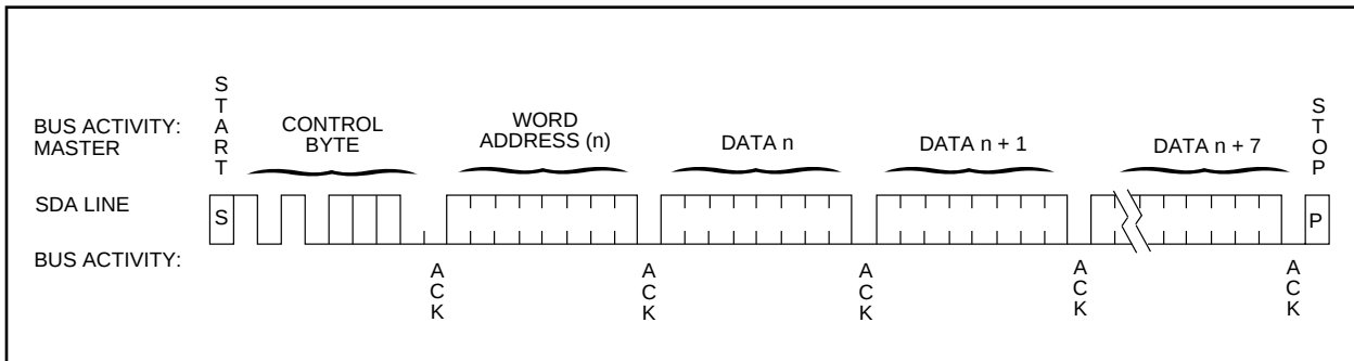
FIGURE 8-1: PAGE WRITE
