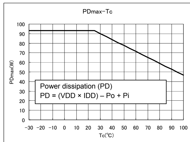
Figure 2 PDmax- T_c
