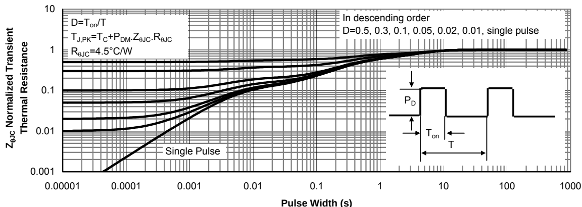
Figure 13: Normalized Maximum Transient Thermal Impedance for AOWF12N60 (Note F)
