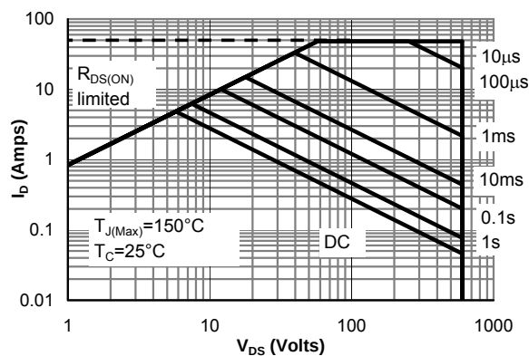
Figure 10: Maximum Forward Biased Safe Operating Area for AOWF12N60 (Note F)
