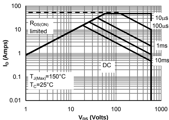
Figure 9: Maximum Forward Biased Safe Operating Area for AOW12N60 (Note F)
