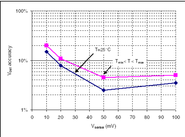
Figure 16. Total output voltage accuracy versus V_{\text{sense}}
