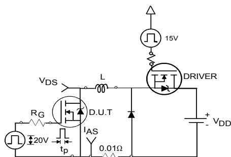
Fig 23a. Unclamped Inductive Test Circuit
