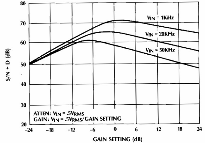
Figure 9. S/N + D vs Gain Setting ( V_{IN}/V_{OUT} = .5V_{RMS} )
