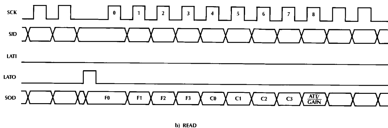
Figure 10. Serial Mode Timing
