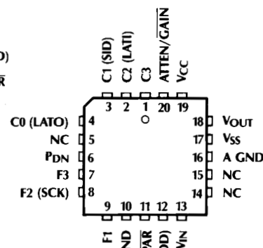
ML2003 20-PIN PCC
