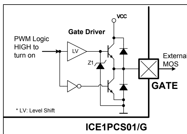
Figure 15 Gate Driver
