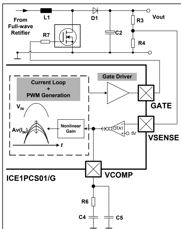
Figure 14 Voltage Loop
