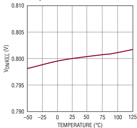
ON/KILL Threshold vs Temperature
