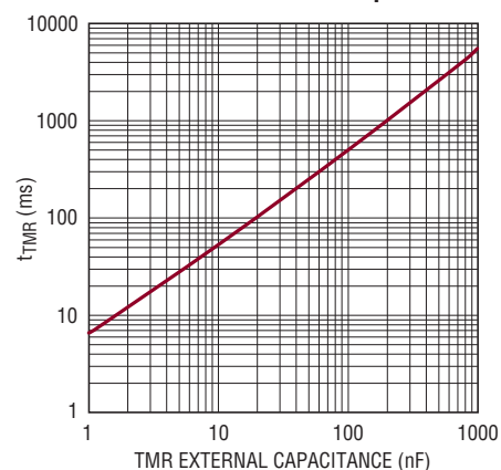
Additional Turn-Off Debounce Time vs TMR External Capacitance
