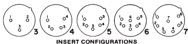
INSERT CONFIGURATIONS
