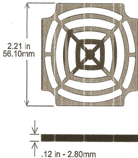
Retainer
