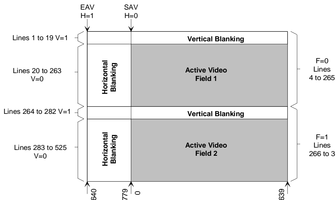
Figure 3. Horizontal and Vertical Timing States (640×480 resolution)
