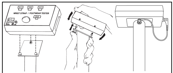
Figure 11. Installing the Combo Tester to the pedestal
