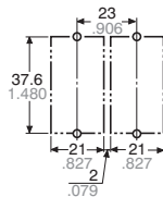
Chassis (Panel) cutout in tandem mounting
