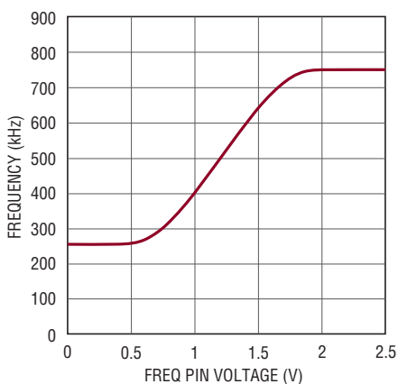
Figure 13. Relationship Between Oscillator Frequency and Voltage at the FREQ Pin
