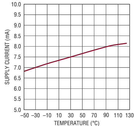
Quiescent Current vs Temperature without EXTVCC
