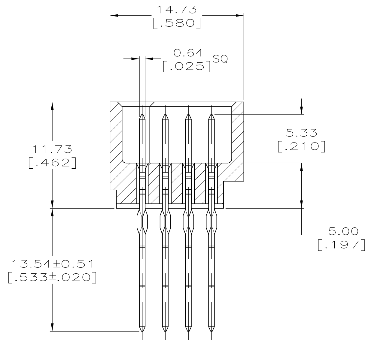
SECTION T-T
