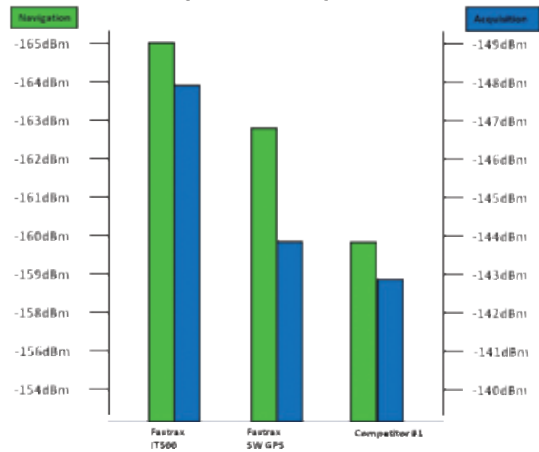
Acquisition and navigation sensitivity comparison of IT500, Fastrax SW GPS and Fastrax main module competitor.
