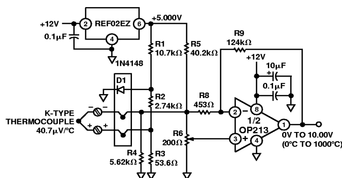
Figure 4. Accurate K-Type Thermocouple Amplifier
