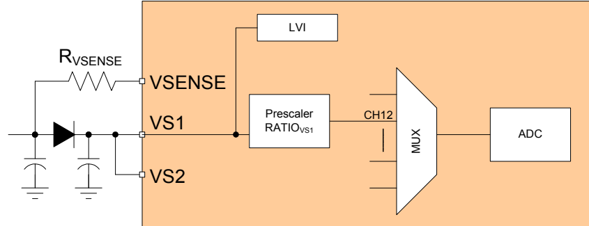
Figure 42. VS1Sense Module
