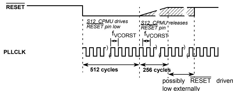
Figure 95. RESET Timing
