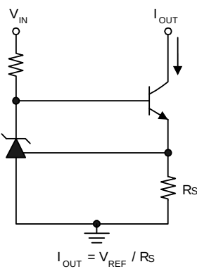
Fig. 7 Constant-Current Sink
