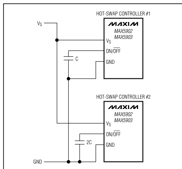
Figure 4. Power-Supply Sequencing
