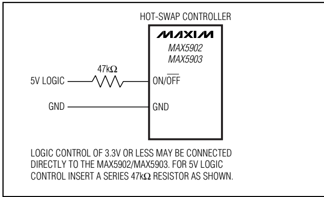
Figure 5. Logic Control
