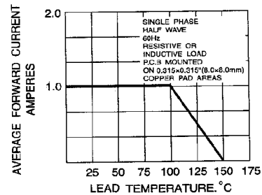
Fig. 2 - MAXIMUM AVERAGE FORWARD CURRENT RATING
