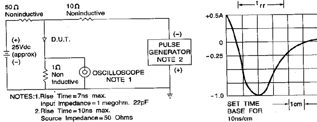
Fig. 1 - REVERSE RECOVERY TIME CHARACTERISTIC AND TEST CIRCUIT DIAGRAM ES1A THRU ES1G
